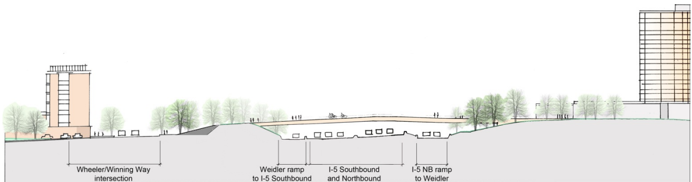
Figure 26: Clackamas Pedestrian/Bicycle Overcrossing, Cross Section (illustrative concept drawing, March 2012)
