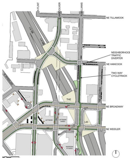
Figure 28: Refined Options North of Broadway (illustrative concept drawings, April 2012)
