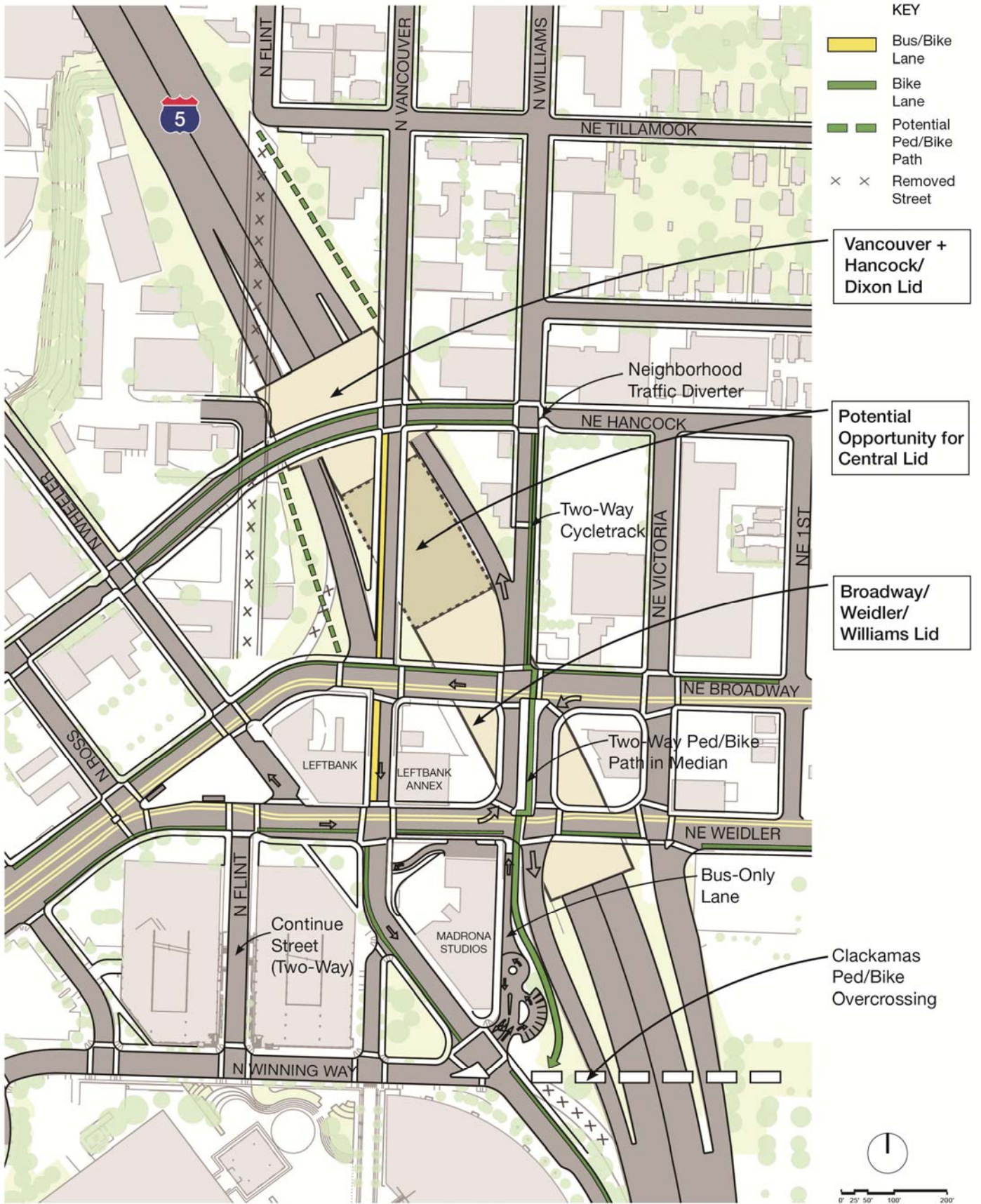
Figure 30: Enlarged “Box” Area of the Recommended Concept
